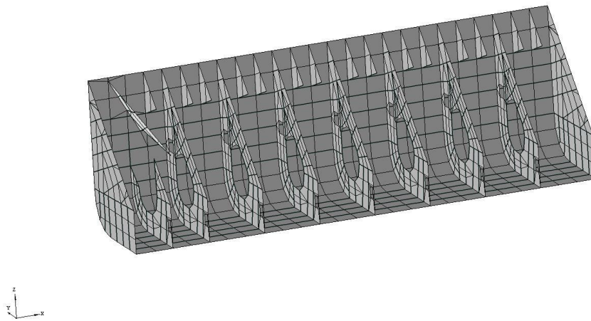
Figure 5: Hopper tanks
